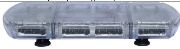
HSM-424 DC12V /DC24V/DC12V-DC24V 1W LED/4pcs LED each module/14pcs modules Size:695*305*98cm (Customized Length) LED/PC Lens:Amber/Red/Blue/Clear/Green
