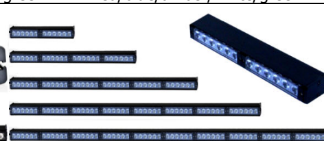
LED Traffic Advisors Lights: HTA-61 DC12V/24V/12V-24V 1W 6LED/LED Module(1-12pcs Optional) Size: 998*50*30mm(8pcs LED Module) red/blue/amber/white/green
