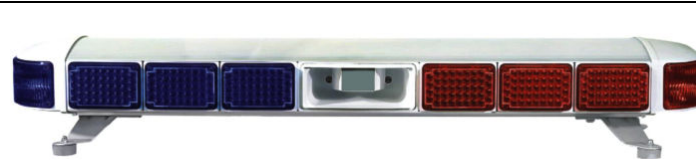
Lightbar HS-1042 DC12V /DC24V/DC12V-DC24V ø5 LED Halogen bulb/ Can With Speaker Full Size:1200*312*165mm (Customized Length) LED:Amber/red/blue/White/Green Aluminum alloy body:Silvery/Black/White
