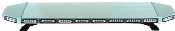
LED Lightbar HS-6140 DC12V /DC24V/DC12V-DC24V 1W or 3W LED/6LED module/22pcs modules/Can with speaker Full Size:121*30*13cm (Customized Length) aluminum alloy body LED:Amber/red/blue/White/Green Body:Silvery/Black/White
