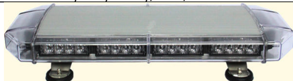
HSM-432 DC12V /DC24V/DC12V-DC24V 1W LED/4pcs LED each module/10pcs modules Size:670*260*85mm (Customized Length) LED/PC Lens:Amber/Red/Blue/Clear/Green aluminum alloy Body:Silvery/Black/White
