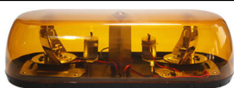
HSM-205 DC12V/DC24V Power:12V-70W/24V-110W/2pcs Halogen bulb Size:590*300*125mm Lens:Amber/Red/Blue/Clear/Green
