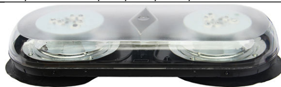
HSM-183 DC12V/DC24V/DC12V-DC24V 3W LED/18pcs LED each Beacon/2pcs Beacons Size:440*200*63mm LED/Lens:Amber/Red/Blue/Clear/Green
