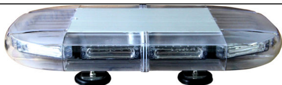
HSM-634B DC12V /DC24V/DC12V-DC24V 1W LED/6pcs LED each module/10pcs modules Size:480*320*100mm (Customized Length) LED/Lens:Amber/Red/Blue/Clear/Green-Body:Silvery/Black/White
