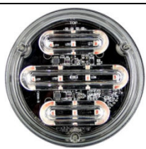
LED Beacon HTL-103 DC12V/24V/DC12-24V 1W /3W LEDs/10pcs Mounting:Bolt Size: Ø124mm*H:28mm Amber,red,blue,White
