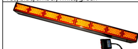
LED Traffic Advisors Lights: HTA-80 DC12V/24V/12V-24V ø5 LED/8pcs LED Modules Size(L/W/H): 830*105*60mm red/blue/amber/white/green
