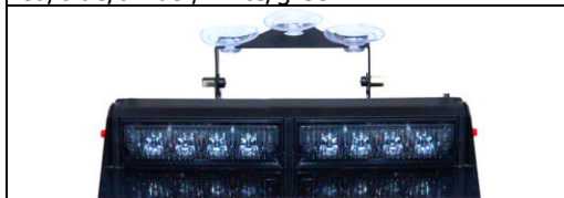
LED Visor Windshield Light: HV-241 DC12V /DC24V/DC12V-DC24V/ 1W LED Size(L/W/H):118mm×143mm×49mm red/blue/amber/white/green
