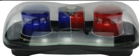
HSM-220 DC12V/DC24V/DC12V-DC24V 1W LED/8pcs LED each Beacon/2pcs Beacons Size:420*207*149mm LED/Lens:Amber/Red/Blue/Clear/Green
