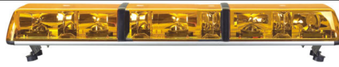
Lightbar HS-1524 DC12V /DC24V/DC12V-DC24V Halogen bulb/Can With Speaker Full Size:1214*296*195mm (Customized Length) PC Dome/aluminum alloy Base Dome Color:Amber/red/blue/White/Green
