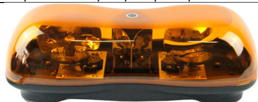
HSM-200 DC12V/DC24V Power:70W/2pcs 35W Halogen bulb Size:420*207*149mm Lens:Amber/Red/Blue/Clear/Green
