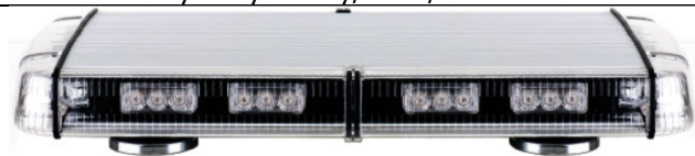
HSM-330 DC12V /DC24V/DC12V-DC24V 1W LED/3pcs LED each module/14pcs modules Size:646*313*87mm (Customized Length) LED/PC Lens:Amber/Red/Blue/Clear/Green Aluminum alloy Body:Silvery/Black/White
