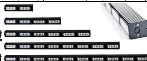
LED Traffic Advisors Lights: HTA-64 DC12V/24V/12V-24V 1W 6LED/LED Module(1-12pcs Optional) Size: 950*55*43mm(8pcs LED Module) red/blue/amber/white/green
