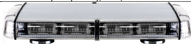
HSM-830 DC12V /DC24V/DC12V-DC24V 1W LED/8pcs LED each module/14pcs modules Size:646*313*87mm (Customized Length) LED/PC Lens:Amber/Red/Blue/Clear/Green Aluminum alloy Body:Silvery/Black/White
