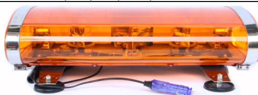
HSM-203 DC12V/DC24V Power:70W/2pcs 35W Halogen bulb Size:500*270*140mm Lens:Amber/Red/Blue/Clear/Green
