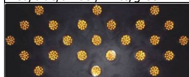
Direction Board: HDB-1580 DC12V/24V/25Set until LED Flash frequency: 60-100n/m Size(L/W/H): 1580*600*90mm red/blue/amber/white/green
