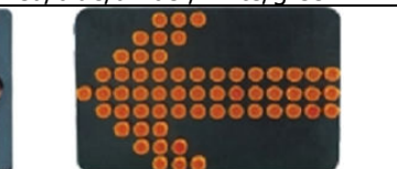
Direction Board: HDB-60 DC12V/24V/58Set until LED Flash frequency: 60-100n/m Size(L/W/H): 600*400*25mm red/blue/amber/white/green
