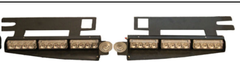
LED Visor Windshield Light: HV-406 DC12V /DC24V/DC12V-DC24V 1 W 4LED/6pcs modules Size(L/W/H):380*230*40mm/1pc red/blue/amber/white/green
